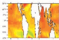
PC1 of CM5 run 3
