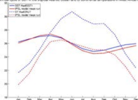
Annual cycle of SST in the tropical Atlantic Ocean and of continental temperature in West Africa region
