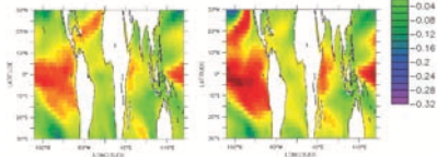
PC1 of CM5 GIG-forced run
