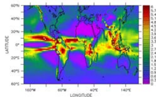
CM5 run 1 stddev
