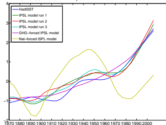
PC 1 of SST trend in the tropics for the model and the observations
