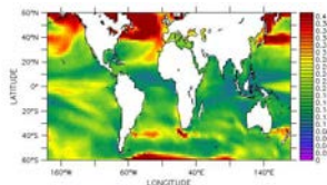
CM5 mean run stddev
