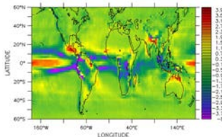
GPCP stddev - run 1 stddev
